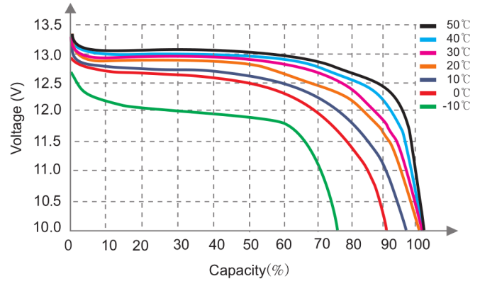
Different Temperature Discharge Curve (0.2C)
