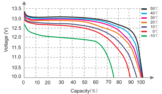
Different Temperature Discharge Curve (0.2C)
